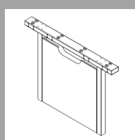
Cable management: • 600 × 50 mm, H: 600 mm • 600 × 80 mm, H: 600 mm
