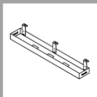
Cable Tray: 900 × 130 mm For front cable access*
